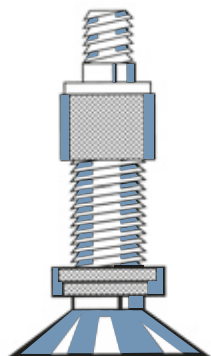
Illustration 29 : Valve Dunlop
