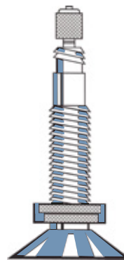
Illustration 30 : Valve Presta
